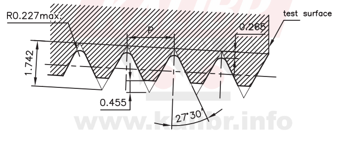
Thread Profile of Ring Gauges.
