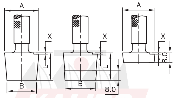
Plain Taper Plug Gauges to check Minor diameter of Internal Threads. (Set of Three Gauges)
