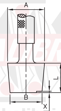
Plain Taper Check Plug for Inspection of Plain Taper Ring Gauge.
